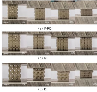
Figure.9. Compression test diagram
