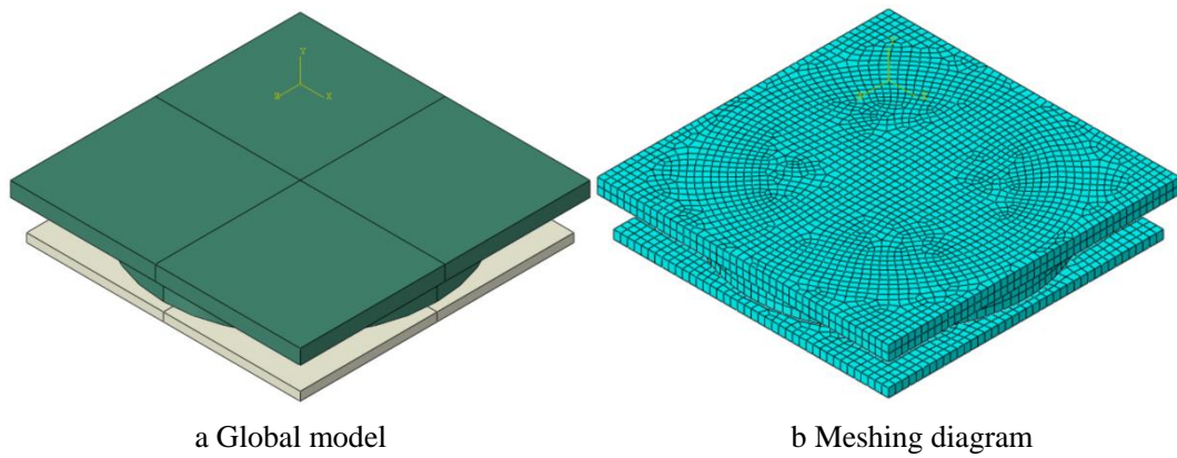
Fig. 2: Finite Element Model of Seismic Spherical Bearing
