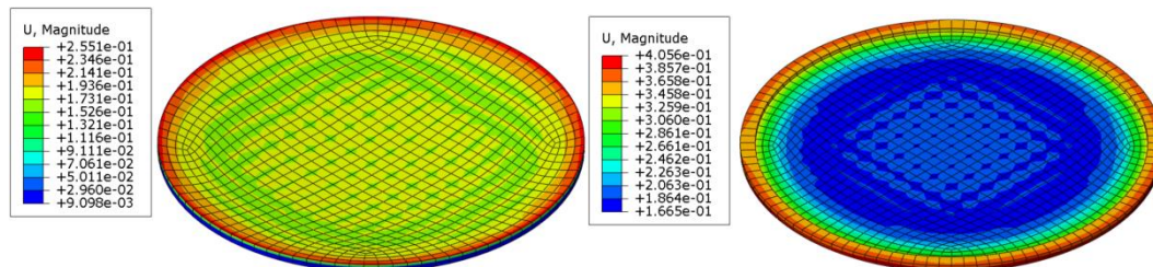
a Strain nephogram of curved PTFE plate
