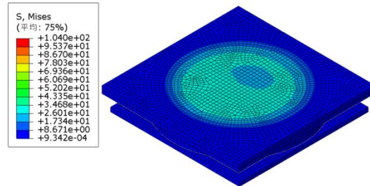
Fig. 6 Mises stress cloud
