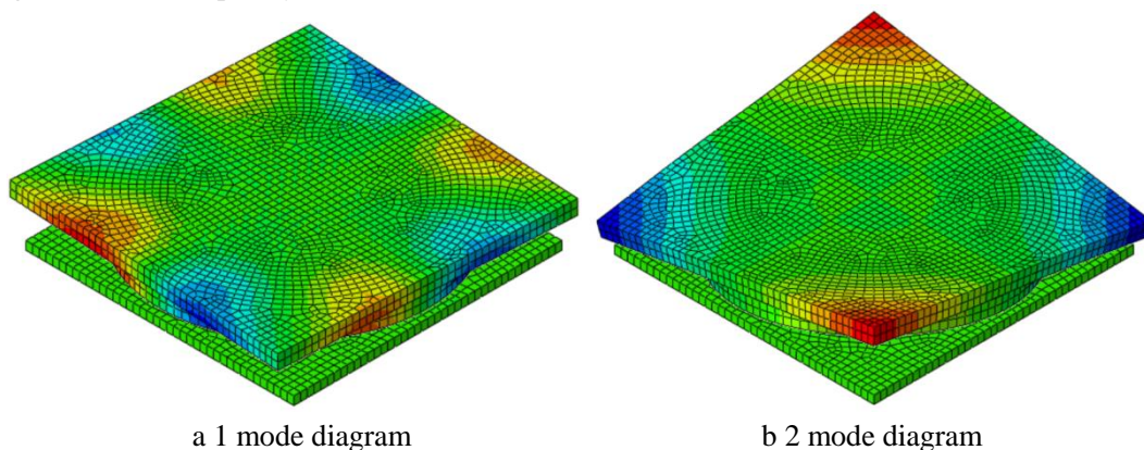
Fig. 7 Vibration Mode Diagram of Bearing
