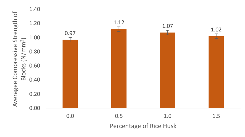
Fig. 2. Average Compressive Strength of Blocks
