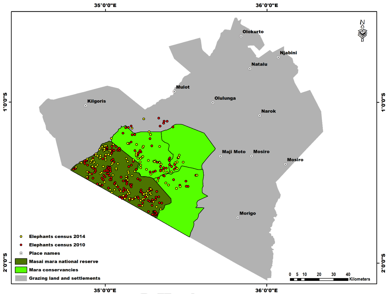
Fig. 3. Distribution of elephants in the MME, Kenya during the 2010 and 2014 aerial censuses
