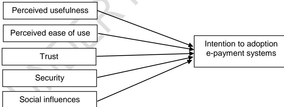
Figure 1: Study's framework
