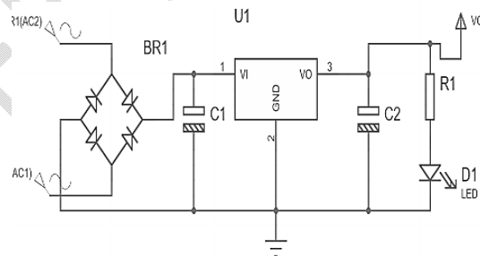
Fig.8 Regulated power supply unit
