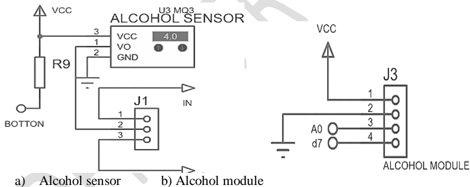
Fig. 2 Alcohol Sensor and Module (Jha 2016)
