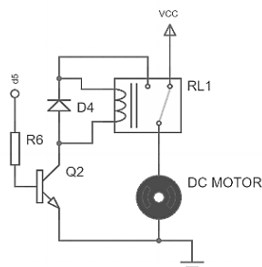
a) Relay output driver
