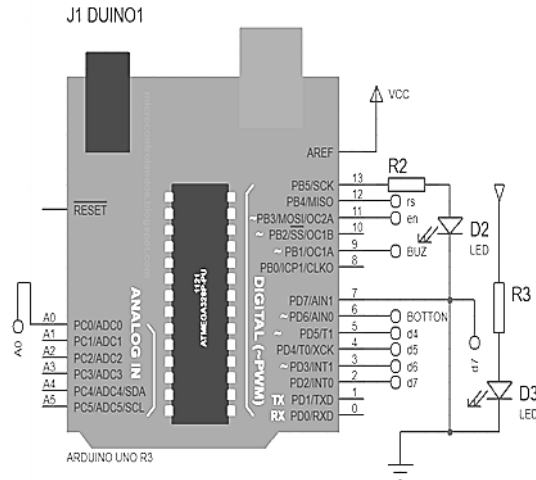
Fig. 7 Microcontroller unit
