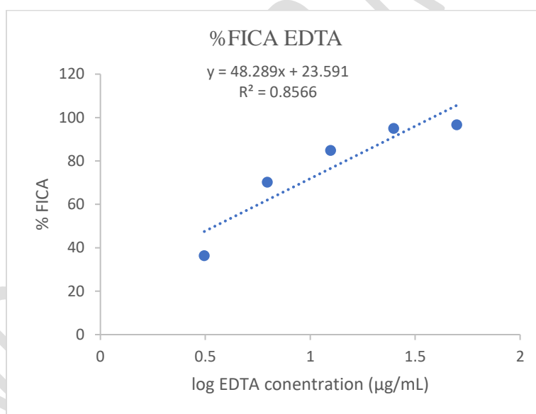
Fig. 4: Chelating power of EDTA IC_{50} = 3.524 \mu\text{g/ml}
