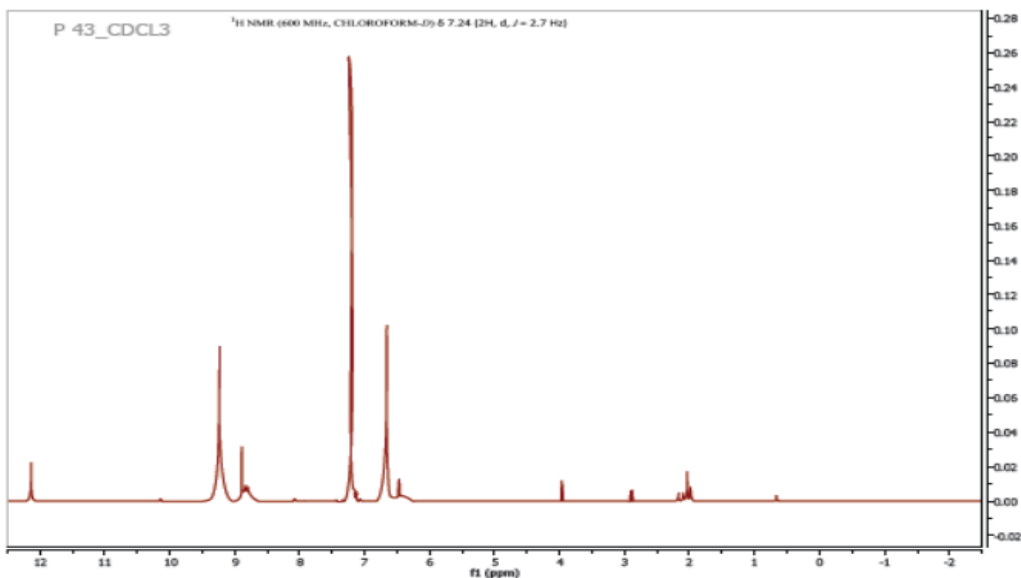
Fig. 8: 1 H NMR of P43
