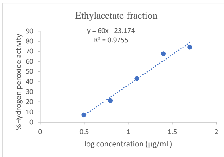
Fig. 5: Ethylacetate fraction \text{H}_2\text{O}_2 activity ( IC_{50} = 16.60 \mu\text{g/ml} )
