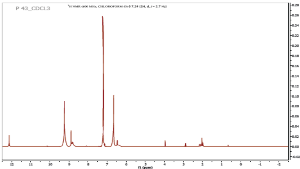
Fig. 8: ^1\text{H} NMR of P43
