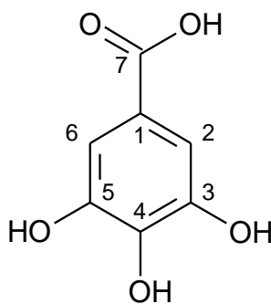
3, 4, 5-trihydroxybenzoic acid (Gallic acid)
