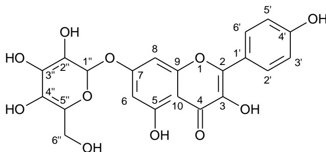
Kaempferol-7-O-glucoside
