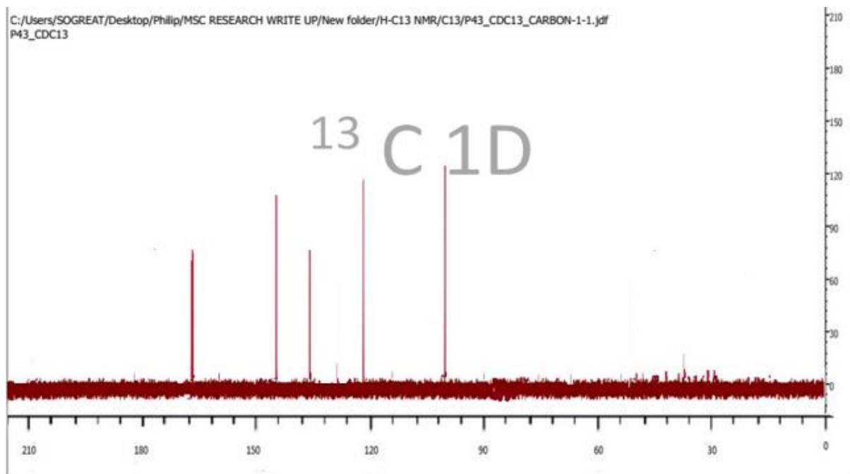
Fig. 9: ^{13}\text{C} NMR of P43
