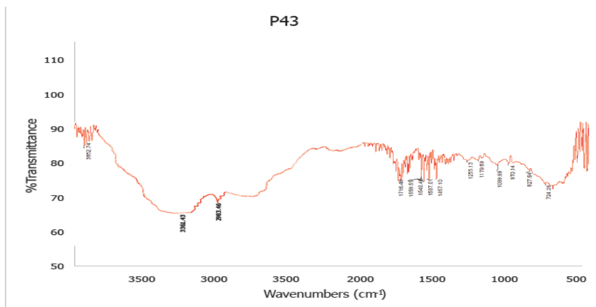
Fig. 7: FT-IR Spectrum of P43
