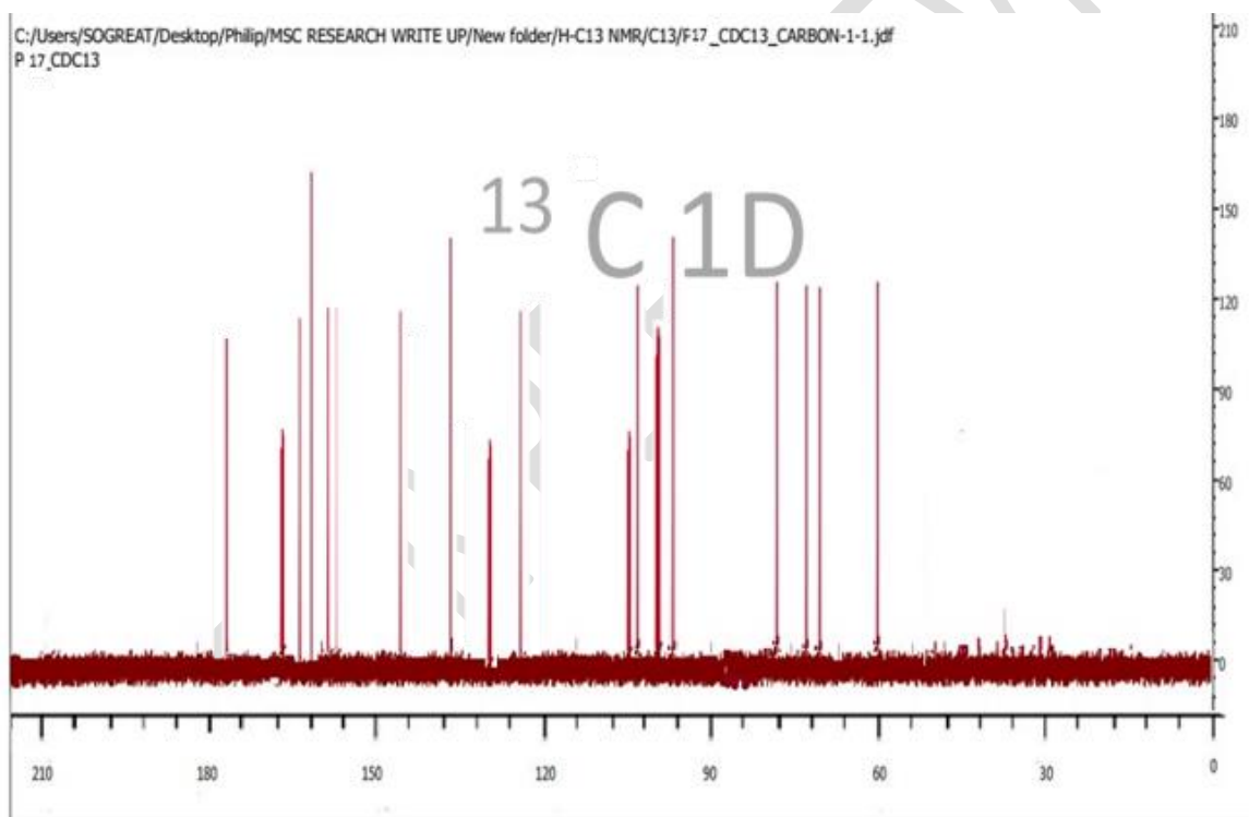
Fig. 12: ^{13}\text{C} NMR Spectrum of P17
