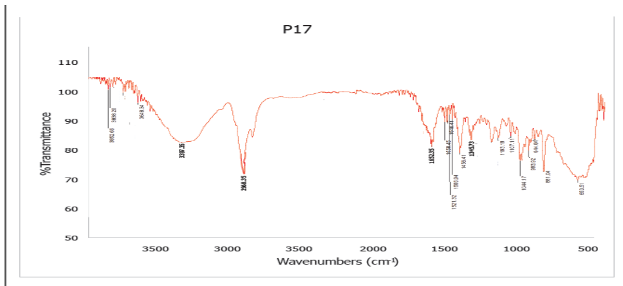
Fig. 10: FT-IR Spectrum of P17
