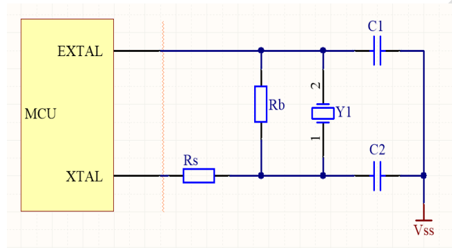
Figure 4 Clock Circuit
