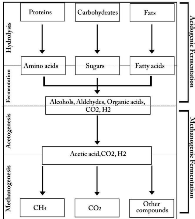
Fig. 1. A schematic of the Anaerobic Digestion process [9].
