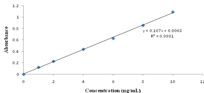
Figure 10B: Linearity graph of CFP using PDAC reagent
