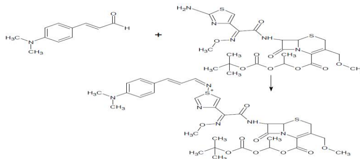
Figure 3: Chromogenic reaction of CFP with PDAC Reagent
