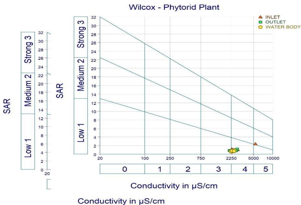
Fig 6. Wilcox Diagram relating EC to Sodium Absorption Ratio (SAR) in Inlet/ Outlet of Phytorid
