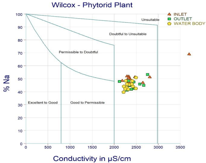
Fig 5. Wilcox Diagram relating EC to % Sodium in Inlet/ and Outlet of Phytorid treatment
