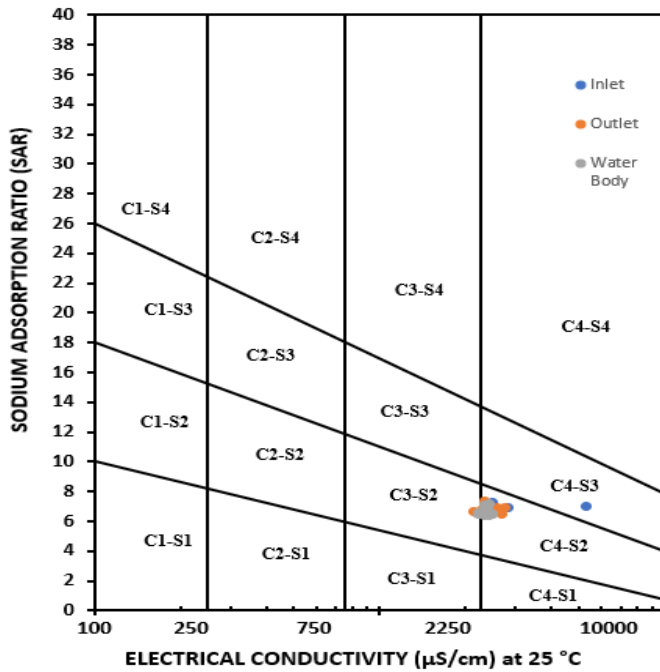
Fig 4. USSL Diagram for Inlet and Outlet of phytorid treatment system at Bindapur
