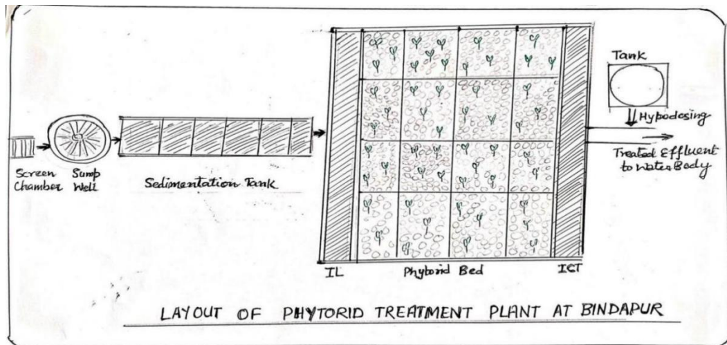
Figure 2: Structural Elements of the Phytorid Treatment System at Bindapur
