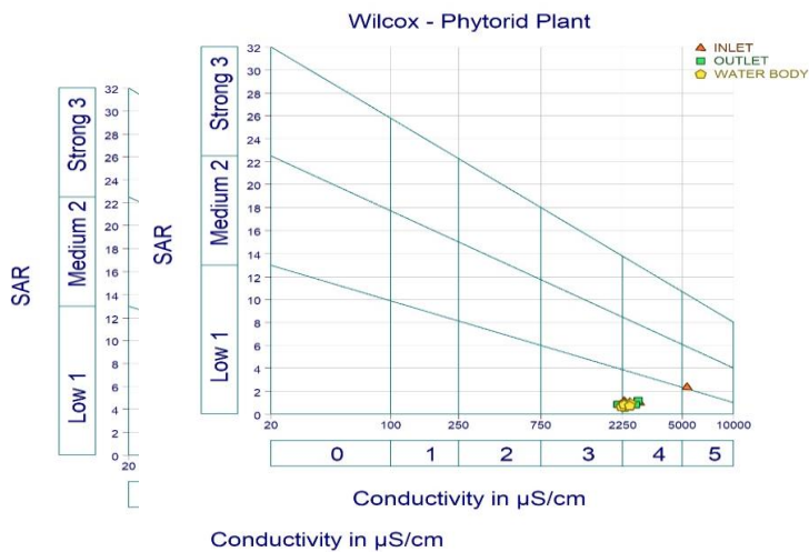
Fig 5 - Wilcox Diagram relating EC to Sodium Absorption Ratio (SAR) in Inlet/ Outlet of Phytorid
