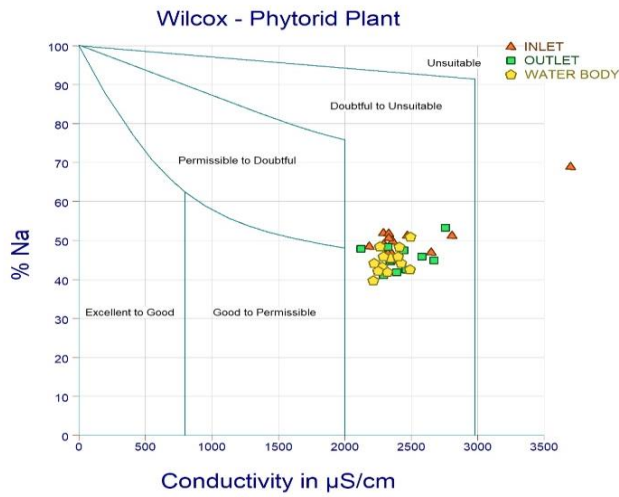
Figure 4 - Wilcox Diagram relating EC to % Sodium in Inlet/ and Outlet of Phytorid treatment
