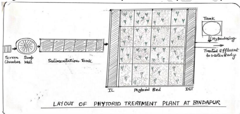
Figure 2: Structural Elements of the Phytoid Treatment System at Bindapur
