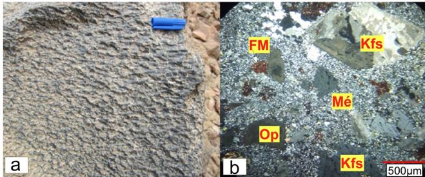
Fig. 8. Aspects of the Mounio trachytes.
