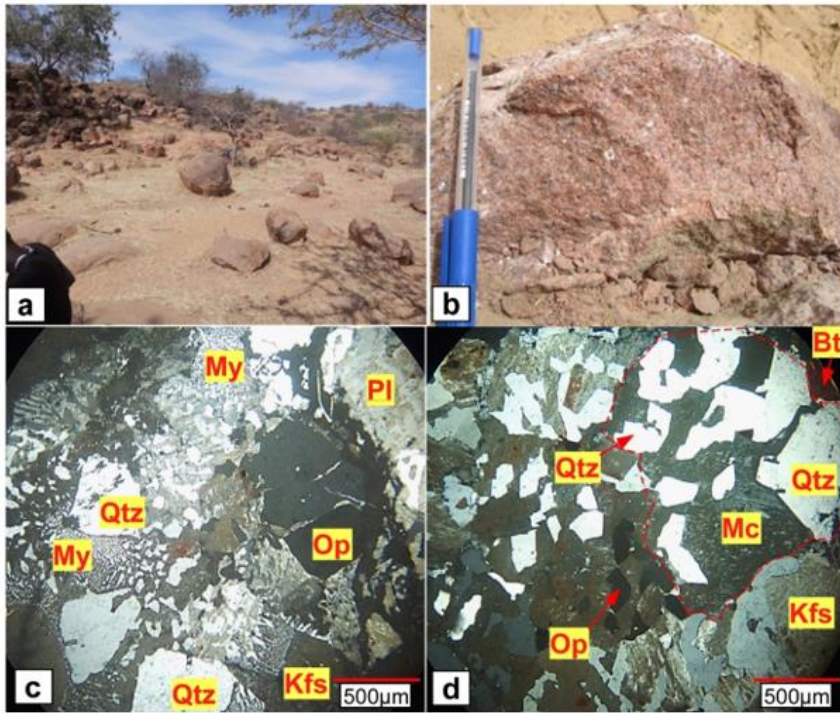
Fig. 11. Mounio quartz syenites.
