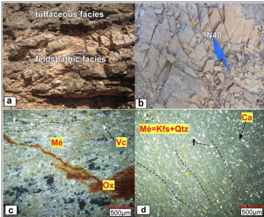
Fig. 5. Aspects of the Mounio metasediments. (a) Metavolcanoclastite with tuffaceous and feldspathic layers; (b) Cataclastic sericite schist; (c and d) Polarised and Analysed Light microphotograph of the Gouré metavolcanoclastite. (b) Cataclastic sericite schist. (c and d) Polarised and analysed light microphotograph of Gouré metavolcanoclastites. [Mé: mesostasis. Qtz: Quartz. Ox: Oxide. Vc: Gas exhaust vacuole. Kfs: Potassium feldspar. Ca: Chalcedony. f: foliation].
