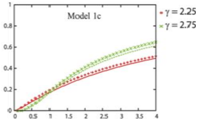
Figure- 2: The density of infected individuals \rho^* is plotted as a function of \lambda for the six different models, when \gamma is 2.25 (red) or 2.75 (green).
