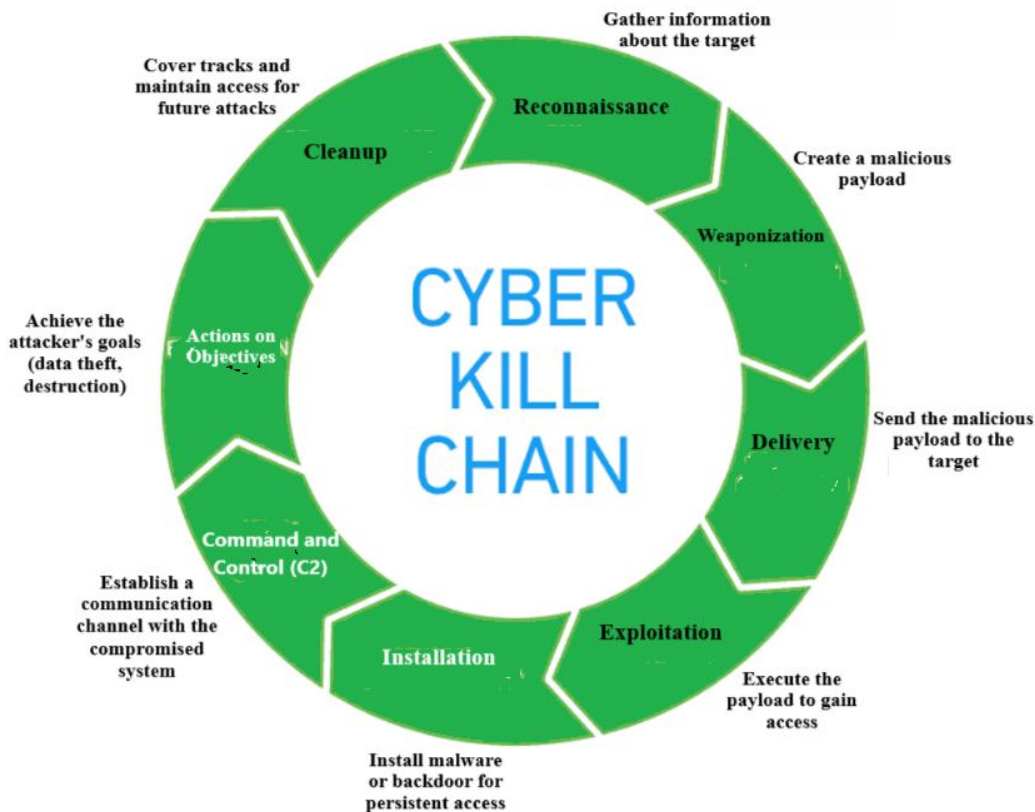
Figure 1: The Cyber Kill Chain Model Source: Developed from Martin (2022)
