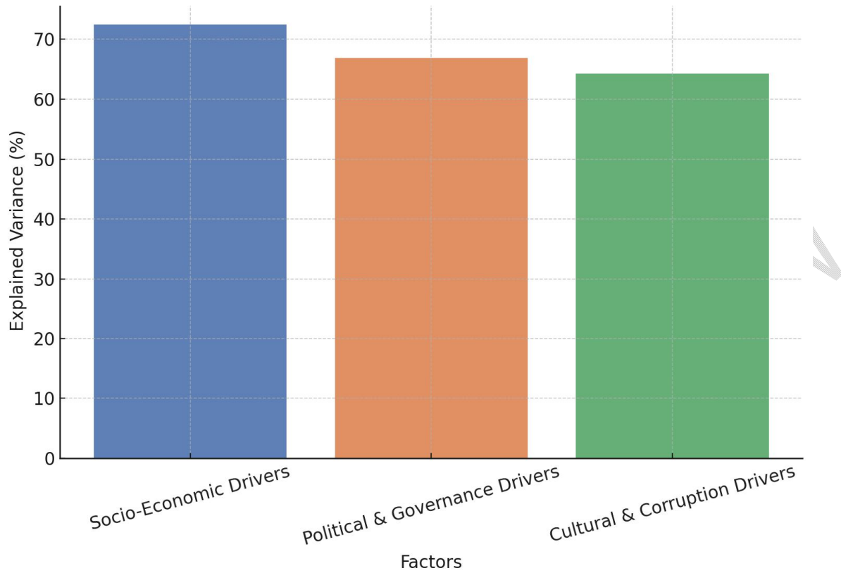
Figure 1: Explained Variance by Factor
