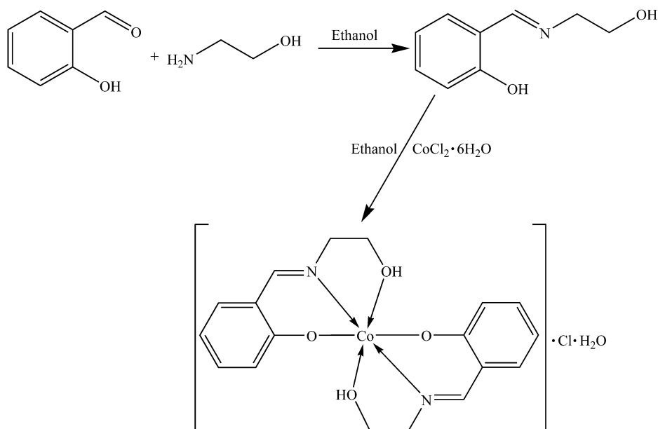
Scheme 1. Synthetic procedure of the ligand H 2 L and the complex [Co(HL) 2 ]-Cl·H 2 O
