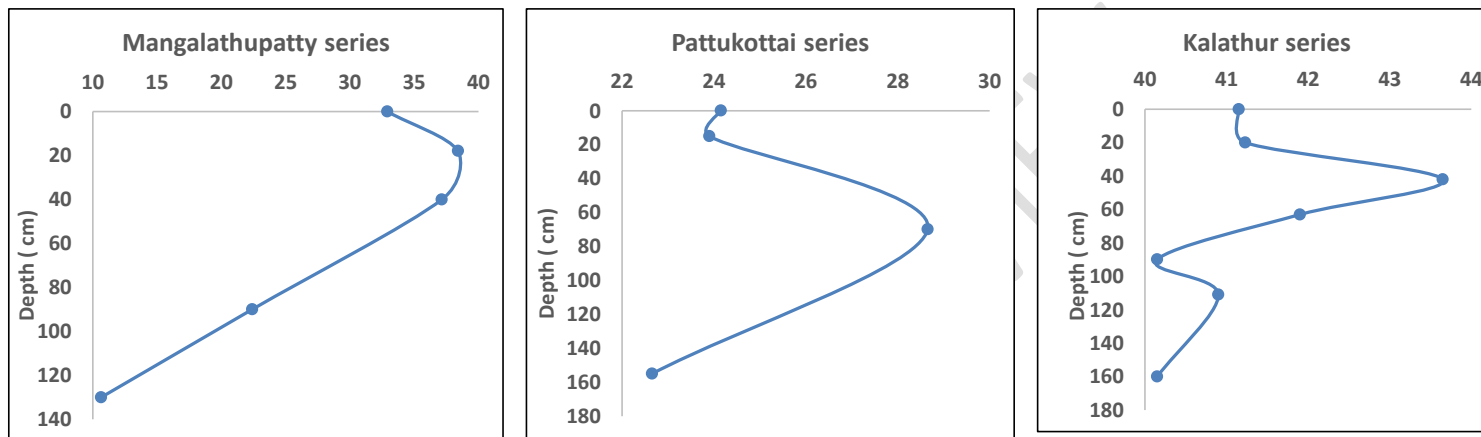
Fig. 1. Distribution of clay in selected soil series of Cauvery Delta zone
