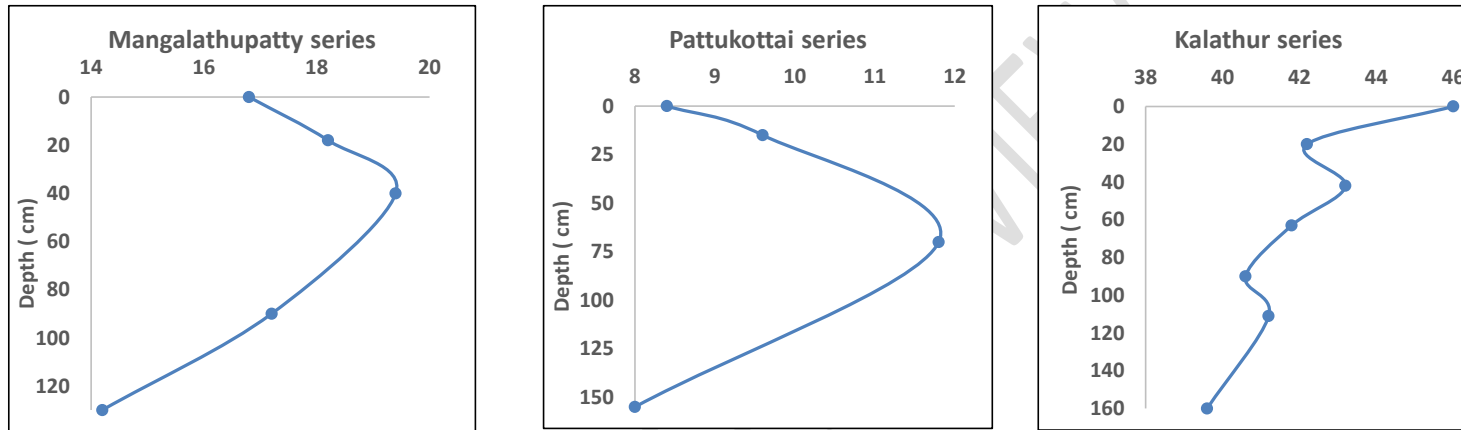
Fig. 2. Cation Exchange Capacity in selected soil series of Cauvery Delta zone
