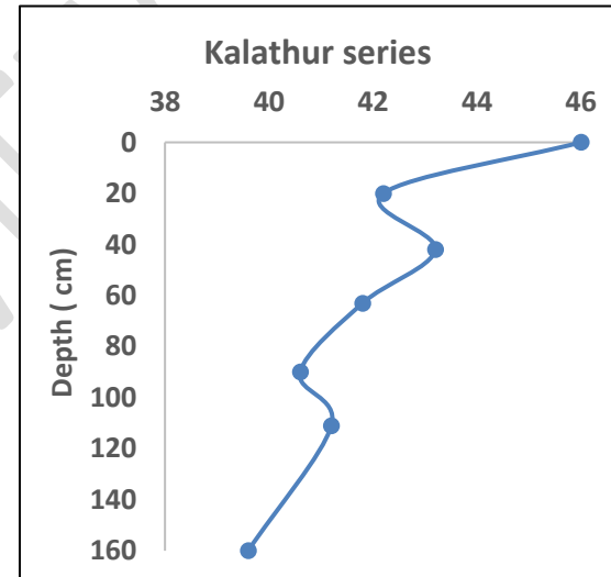
Fig. 2. Cation Exchange Capacity in selected soil series of Cauvery Delta zone
