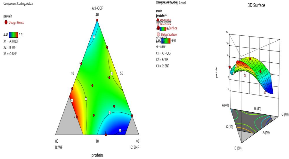
Figure 13. Contour and 3D surface plots of protein content (%) for composite cassava-wheat-bambara bread
