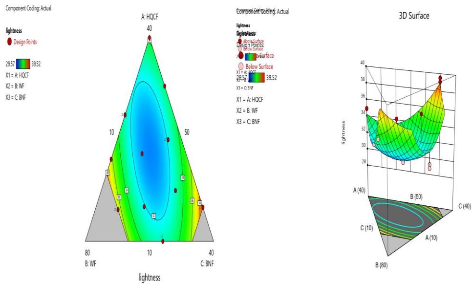
Figure 1. Contour and 3D surface plots of lightness for composite bread from blends of HQCF, wheat flour and Bambara nut flour
