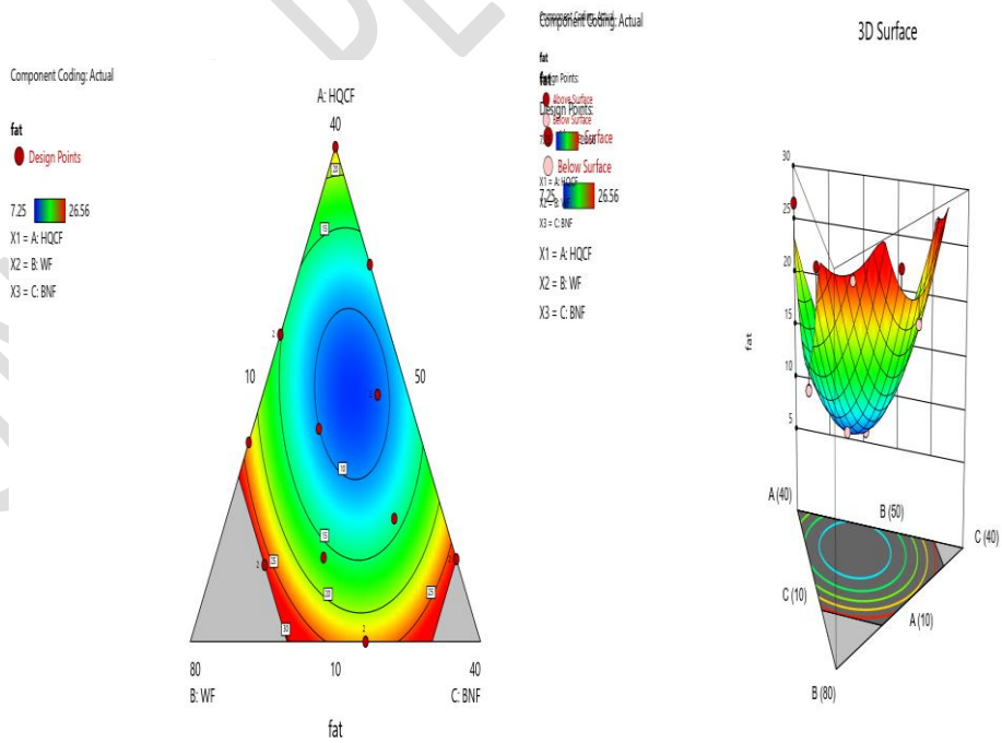
Figure 12. Contour and 3D surface plots of fat content (%) of composite cassava-wheat-bambara bread
