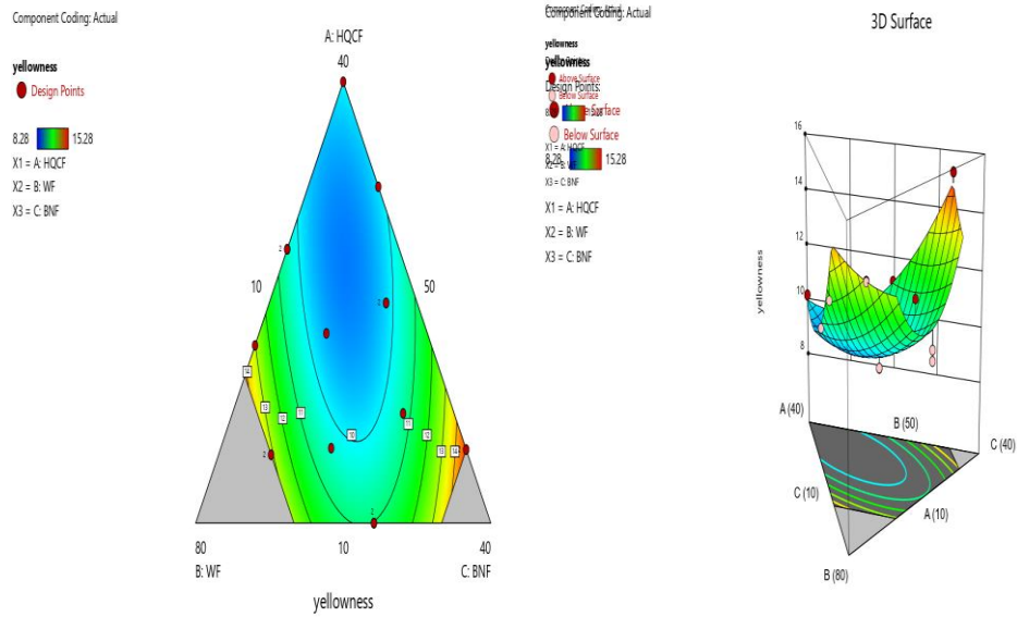
Figure 3. Contour and 3D surface plots of yellowness for composite bread from blends of HQCF, wheat flour and Bambara nut flour
