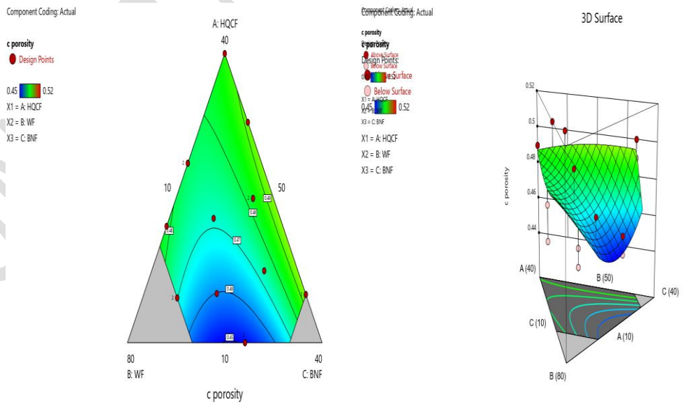
Figure 6. Contour and 3D surface plots of crumb porosity for composite bread from blends of HQCF, wheat flour and Bambara nut flour
