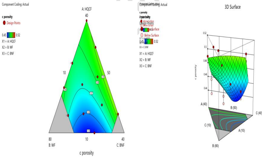
Figure 6: Contour and 3D surface plots of crumb porosity of composite bread from blends of HQCF, wheat flour and Bambara nut flour
