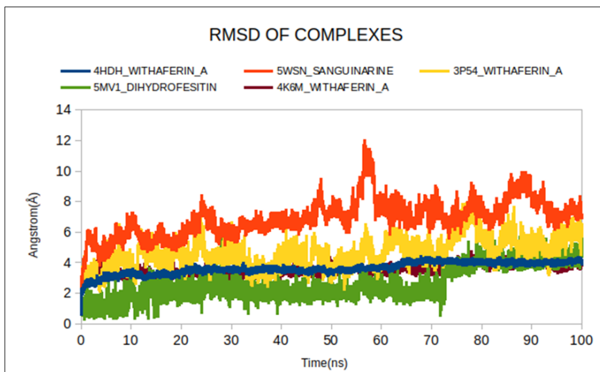
Figure 3: Root mean square deviations of complexes
