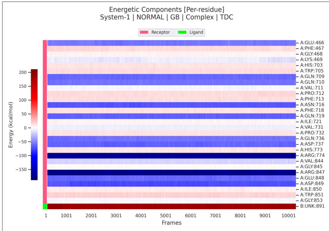
Figure 10: GB Decomposition Energies for the complex
