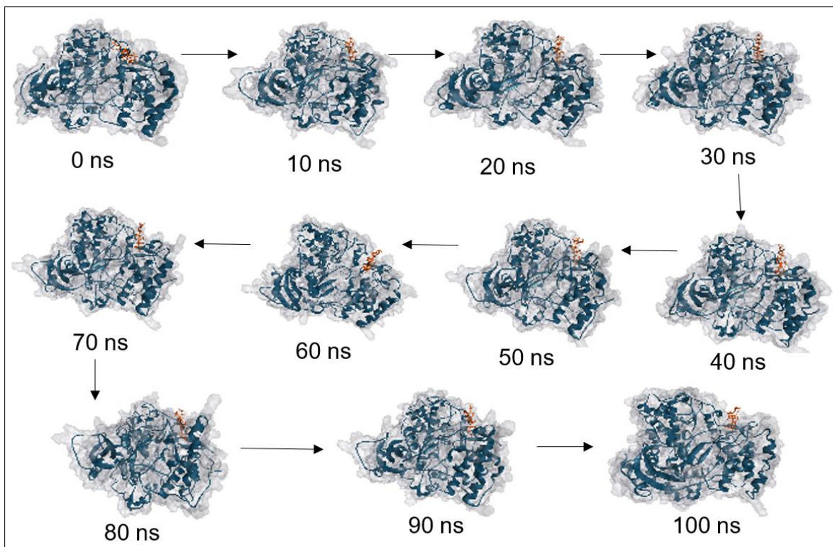
Figure 12 Visualization of Trajectory of 4HDH_WithaferinA
