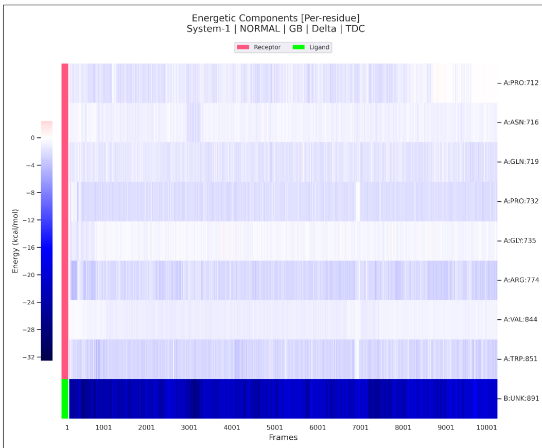
Figure 11: GB Delta decomposition for the complex
