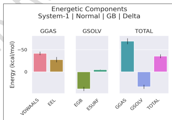
[4HDH_withaferin A]
