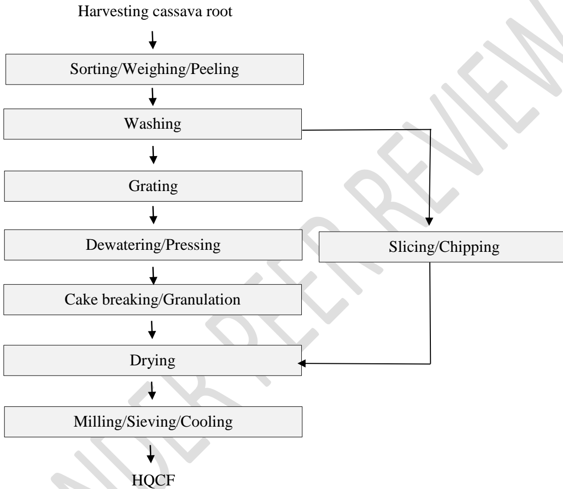
Figure 1. Flow chart for the production of high quality cassava flour
