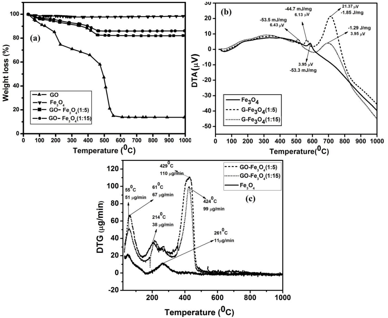
Figure 4: TGA, DTA and DTG graph of GO and GO-Fe 3 O 4 nanocomposites
