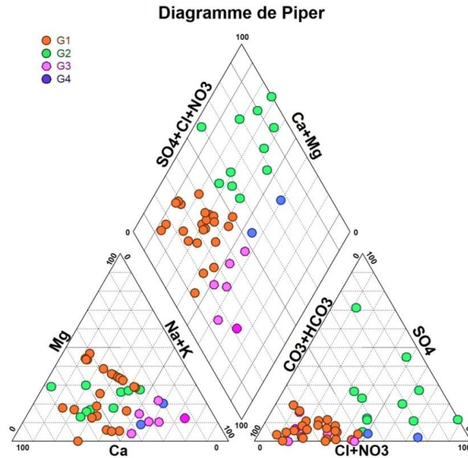
Figure 4: Piper Trilinear diagram
