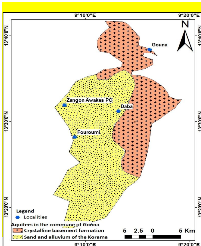
Figure 2: Geological map of the commune of Gouna
