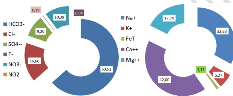
Figure 3: Descriptive statistics for physico-chemical water parameters
