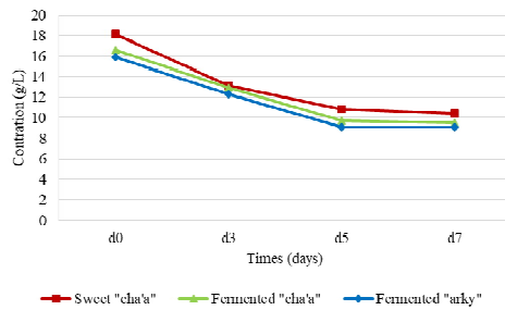
Figure 3. Evolution of reducing carbohydrates concentrations with time
