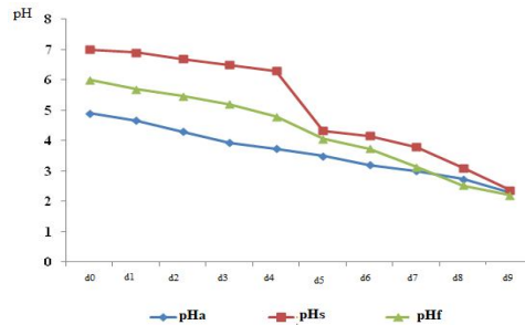
Figure 2. Evolution of pH values with time pHa: pH in fermented "arky" juice; pHs: pH in fresh sweet "cha'a"; pHf: pH in fermented "cha'a"
