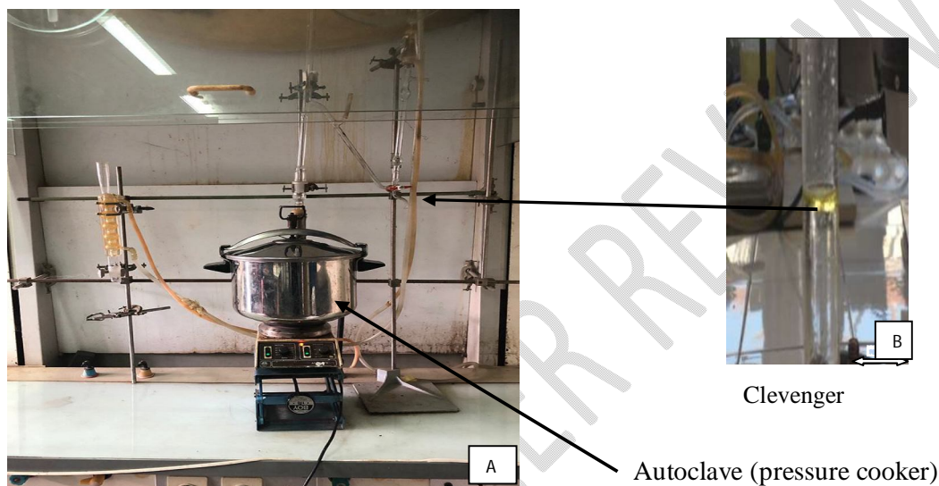
Figure 2: A. Autoclave (Using Pressure cooker) and B. Clevenger devices for extracting essential oils (Atché photos: 24/08/2019)
