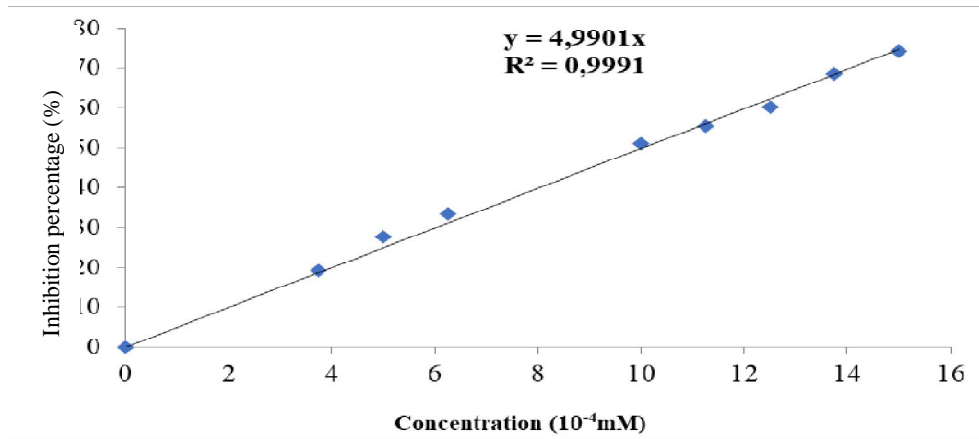
Figure 7 :Trolox calibration (ABTS)
