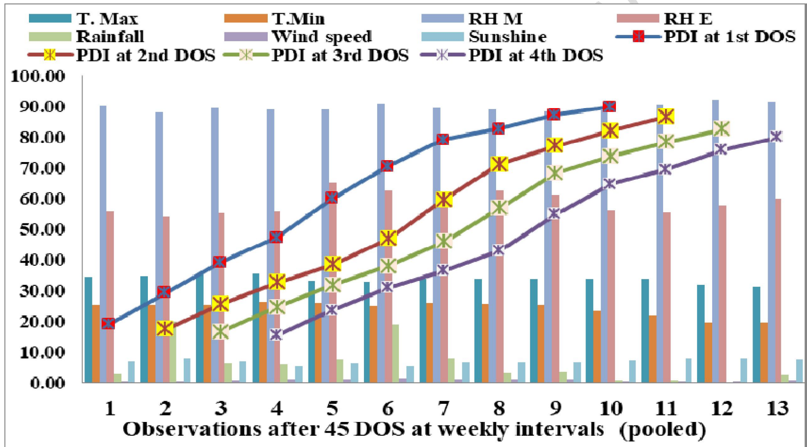
Figure 1: Progression of maydis leaf blight disease incidence in relation to weather parameters in different date of sowing during Kharif -2021 and 2022 (Pooled).
