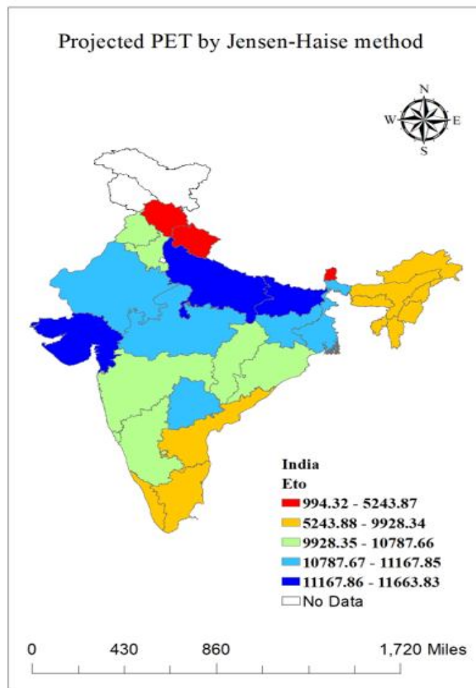
Fig. 3. Spatial variation in mean annual PET across India for the projected 50 years (2021-2070)
