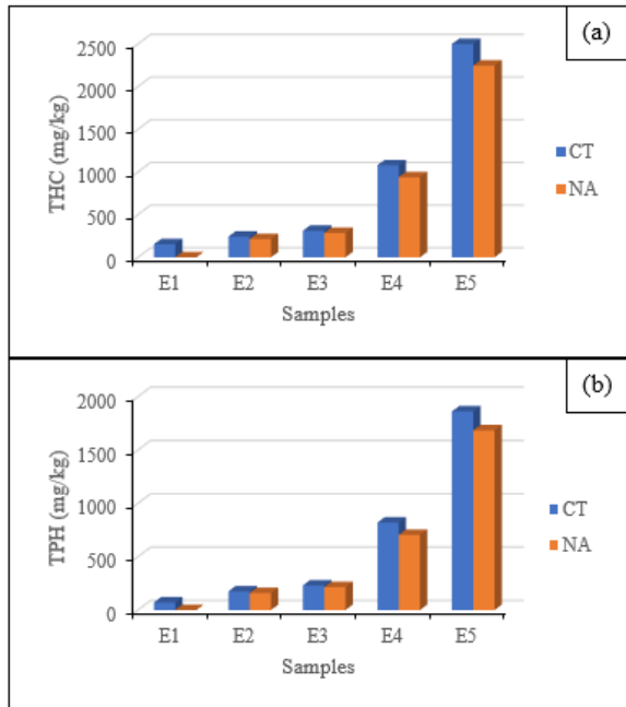
Figure 2: Comparison of THC and TPH of contaminated and natural attenuation of Elele soil
