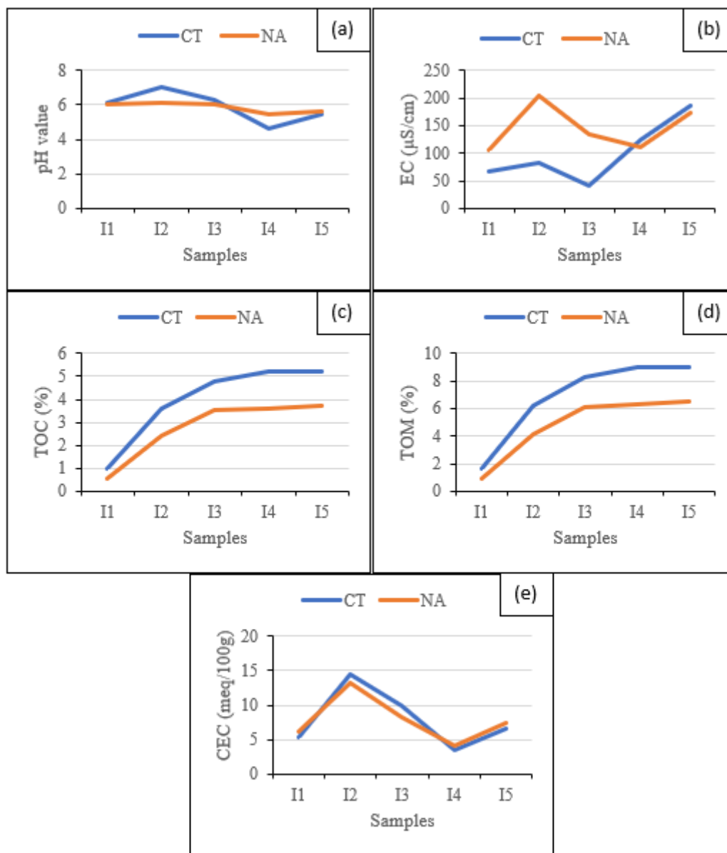
Figure 5: Comparison of physicochemical properties of contaminated and natural attenuation of Isiokpo soil
