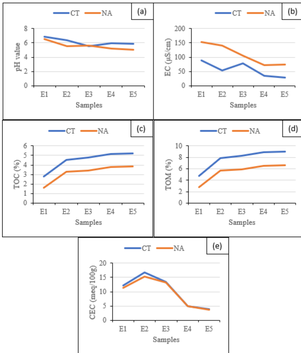
Figure 4: Comparison of physicochemical properties of contaminated and natural attenuation of Elele soil
