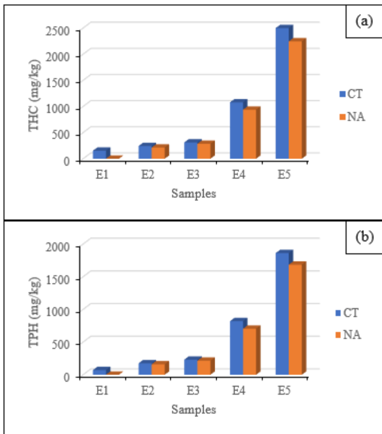
Figure 2: Comparison of THC and TPH of contaminated and natural attenuation of Elele soil
