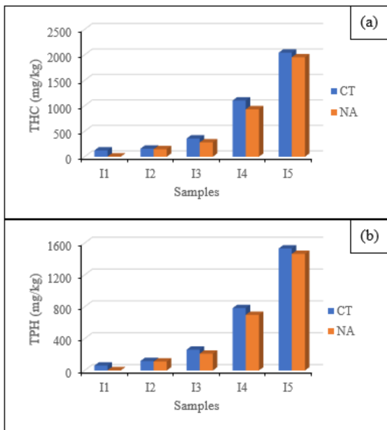
Figure 3: Comparison of THC and TPH of contaminated and natural attenuation of Isiokpo soil
