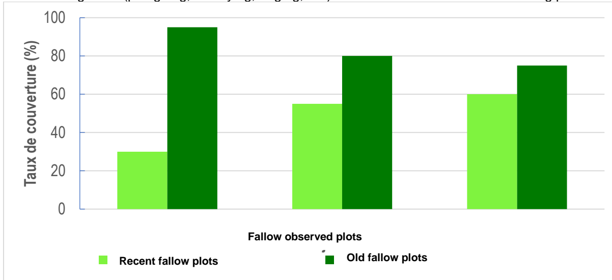
Figure 10 : Temporal evolution of the coverage rate of biological crusts on fallow plots
