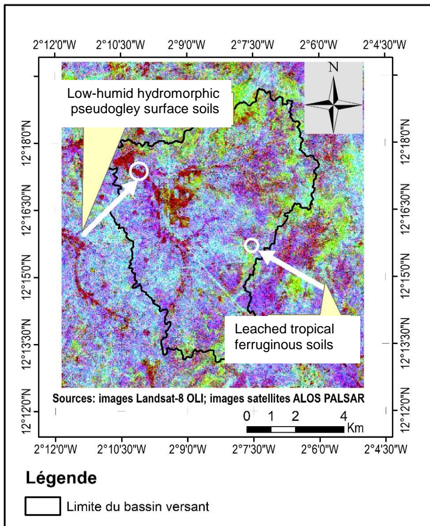
Figure 5 : Colored composition of Landsat-8 OLI satellite image indexes
