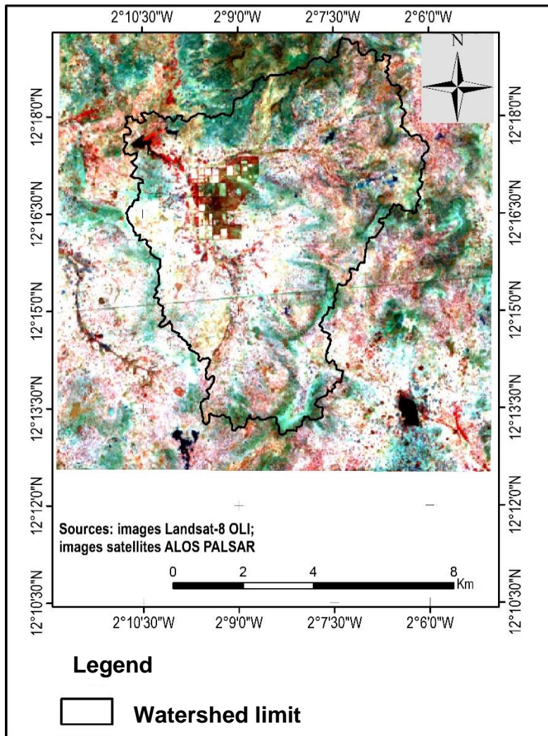
Figure 7 : Land cover units in the Saria watershed
