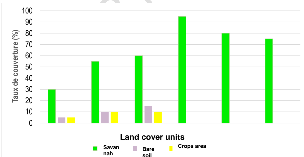
Figure 9 : Biological soil crusts on soils units
