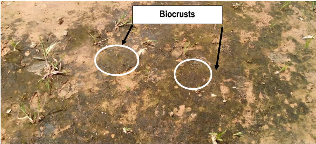
Figure 2 : Soil biological crusts
