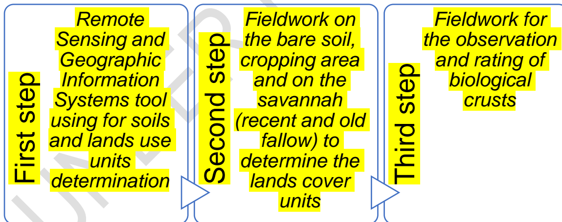
Figure 4 : Workflow on the essential steps of the methodology
