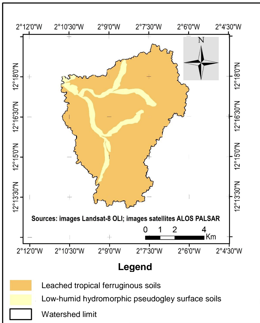
Figure 6 : soil types in the Saria
