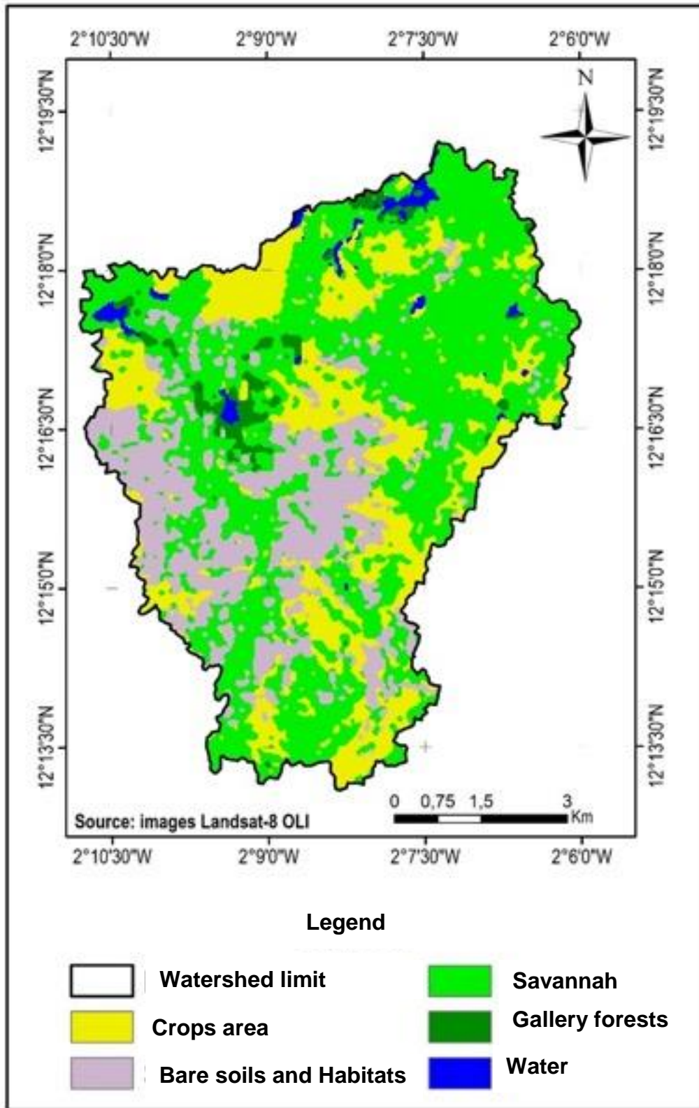
Figure 8 : Land use units in the Saria watershed
