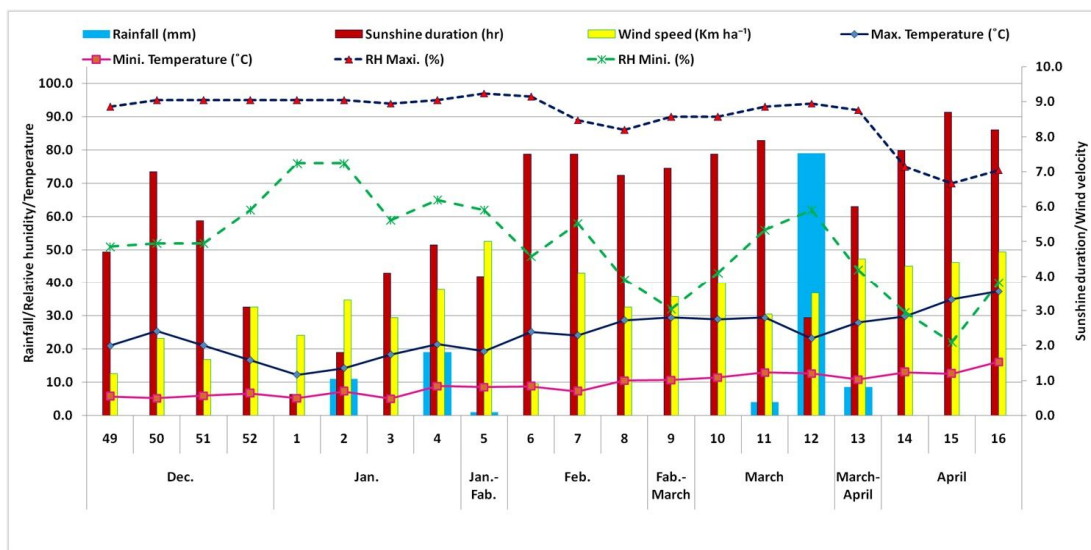
Fig.1 Mean weekly meteorological observation during crop season
