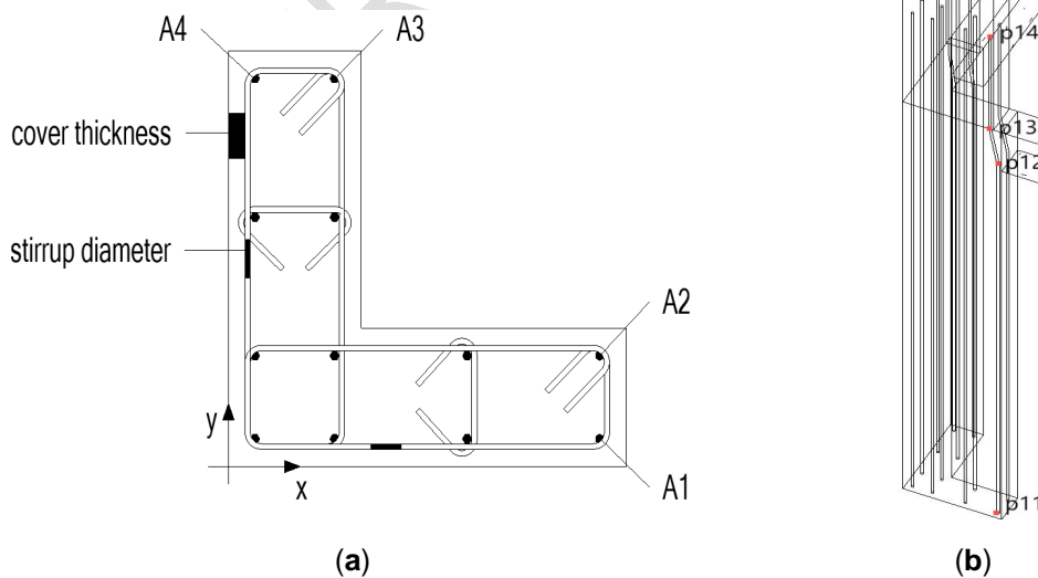
Figure 6. (a)Schematic diagram of column limb longitudinal rebar; (b)Locating points for longitudinal rebar A1
