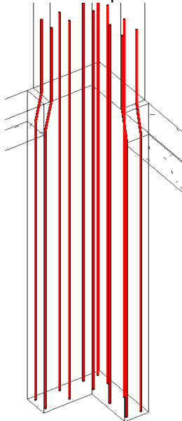
Figure 7. 3D view of longitudinal rebar of L-column
