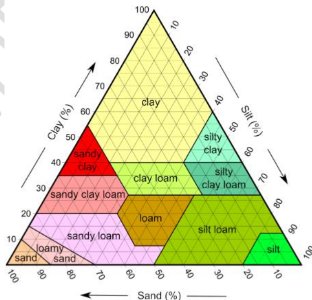
Fig. 2. Soil texture triangle diagram [17]
