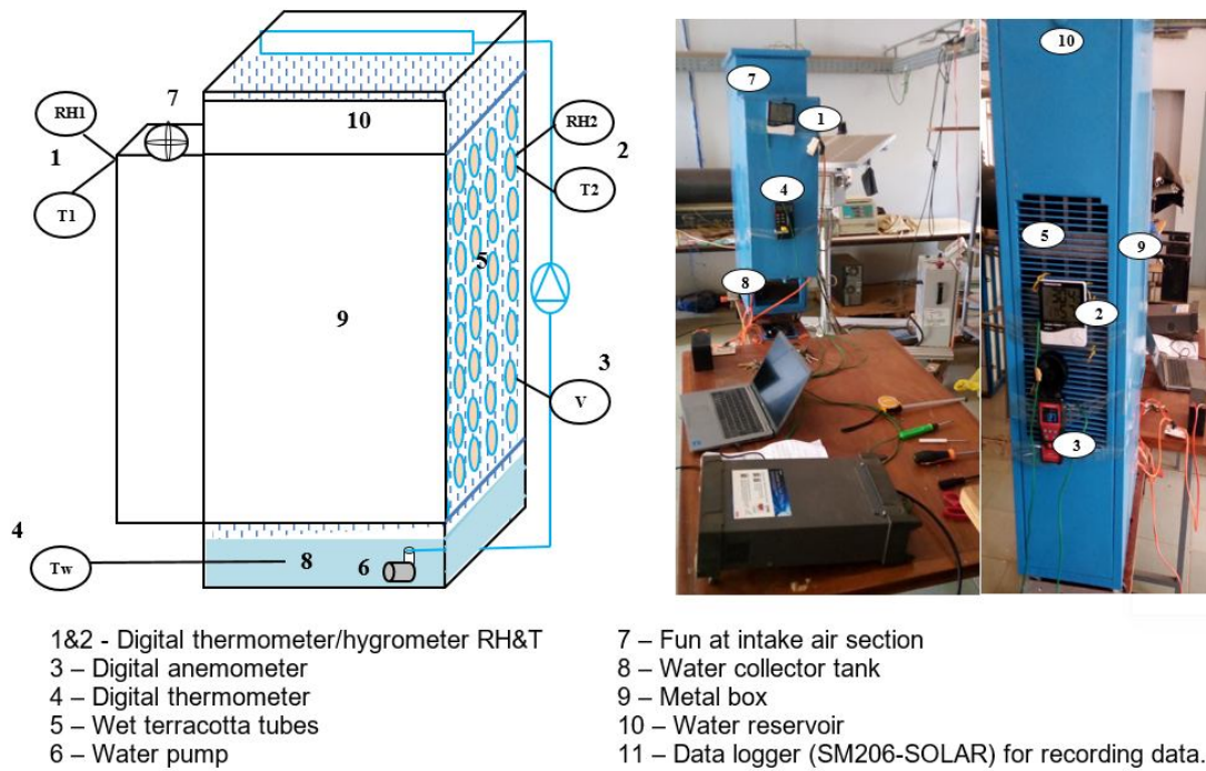
Figure 4: Experimental setup
