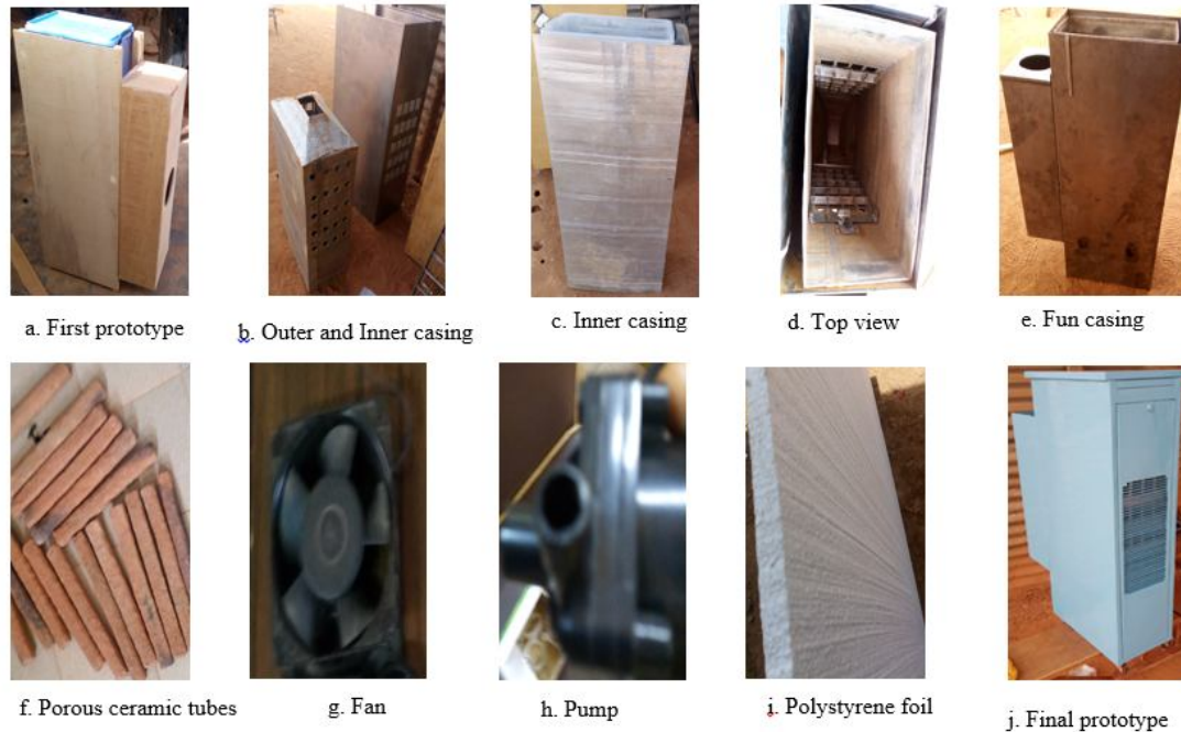
Figure 3: Prototype assembly components
