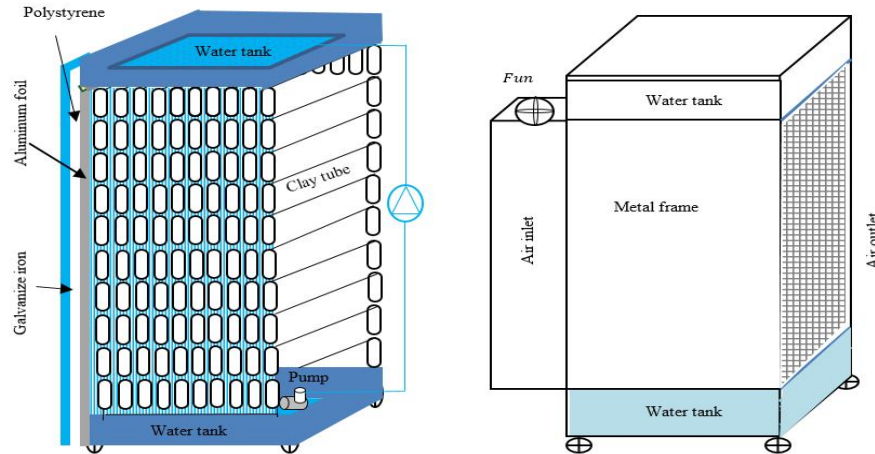
Figure 1: Prototype of the terracotta tube evaporative cooler
