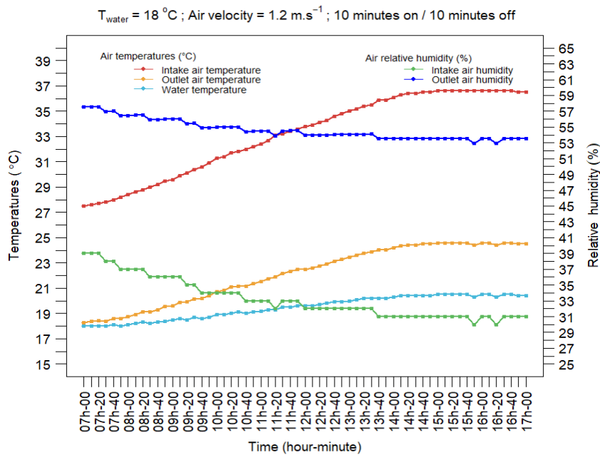
Figure 8: The dynamic operating performance of the cooler
