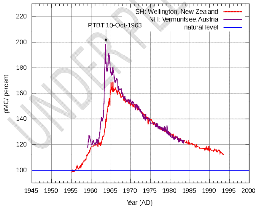
Fig. 2: 14 CO 2 concentration in the atmosphere: Pulse and decay after the atomic bomb tests [29].
