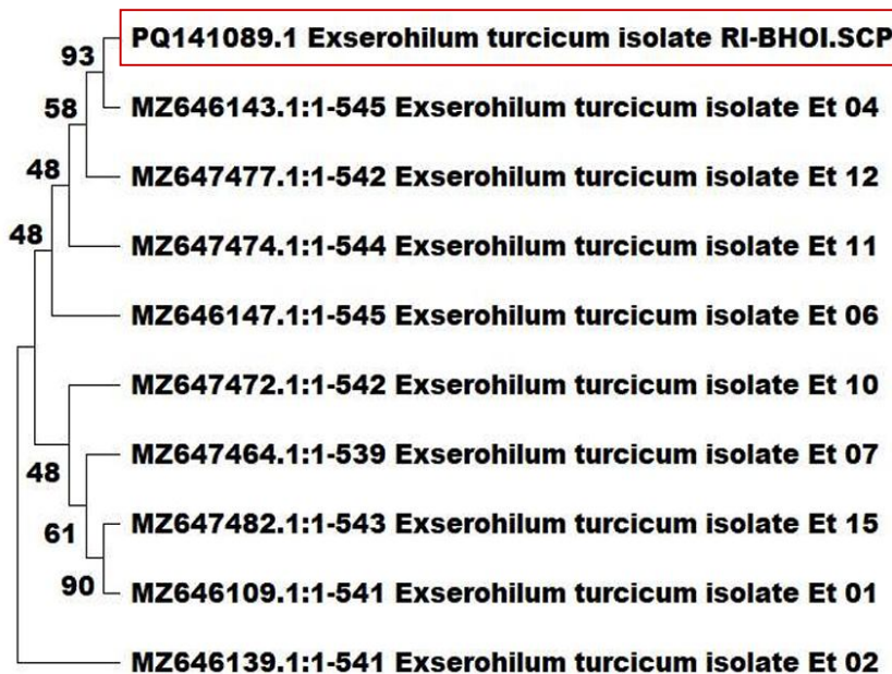
Fig. 8: Phylogenetic tree based on the maximum likelihood method analysis of the ITS rDNA region for Exserohilum turcicum isolate and their closest taxa (Numbers at the nodes indicate the bootstrap values from 1,000 replications)
