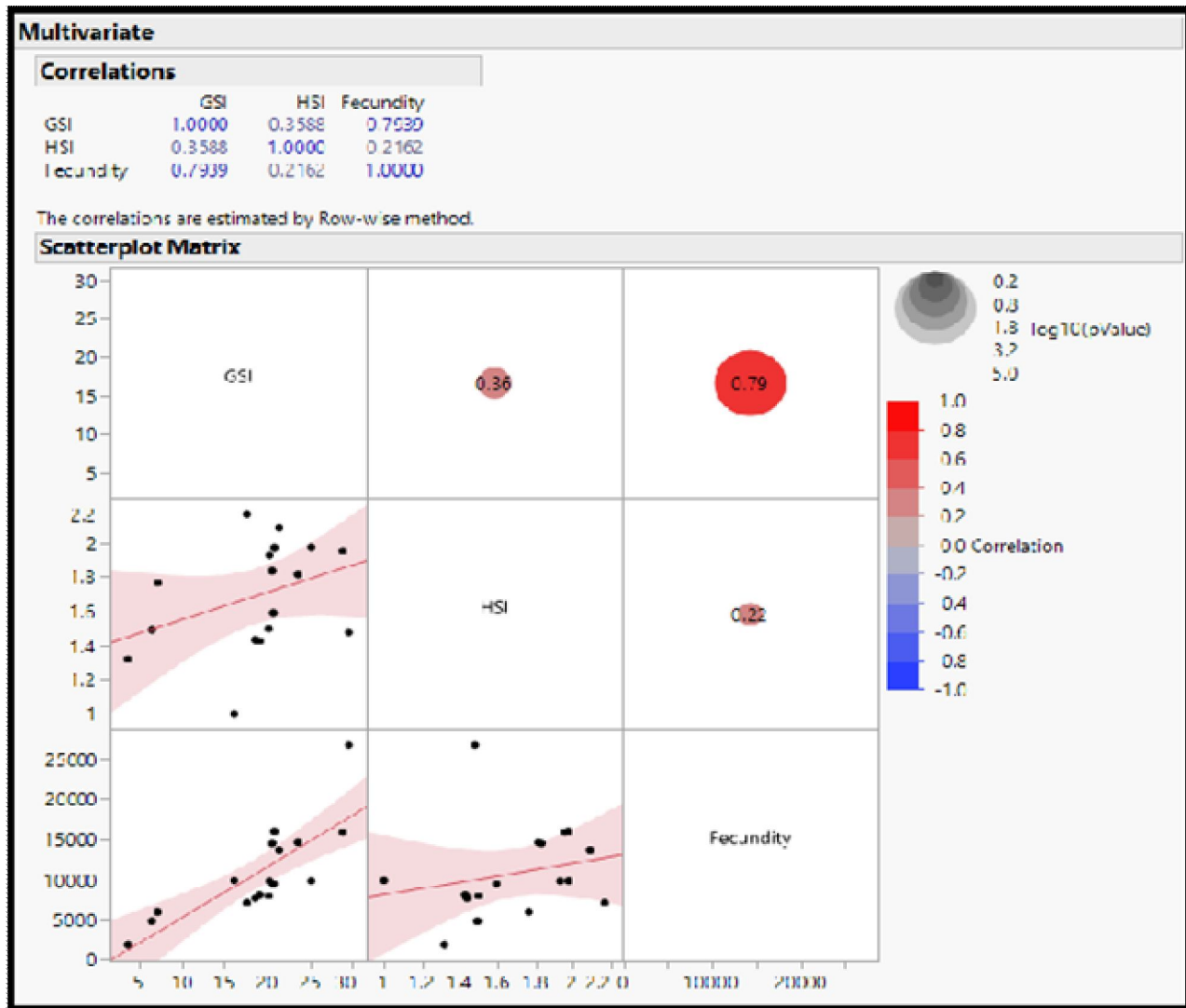
Fig. 8: Correlation and Scatterplot Matrix
