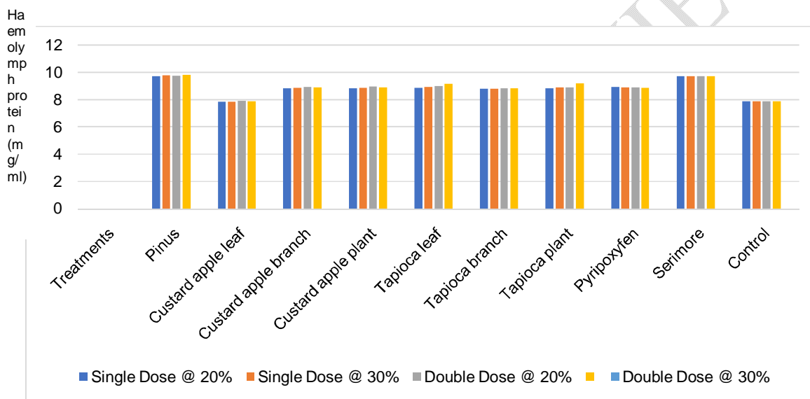
Fig.1. Effect of different Juvenile hormone mimics on haemolymph protein of silkworm B. mori L.
