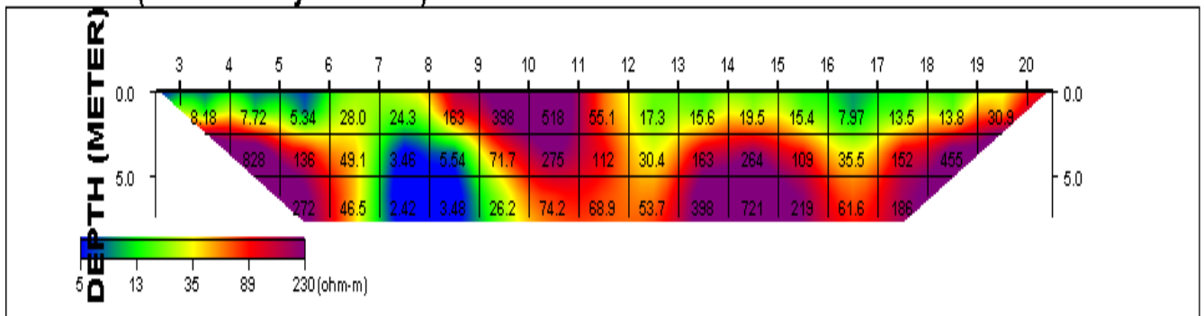
Traverse 2 (2-D Resistivity Structure)
