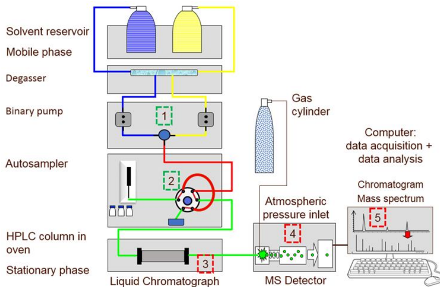
Figure 4: LC-MS (Source: Technology Networks)
