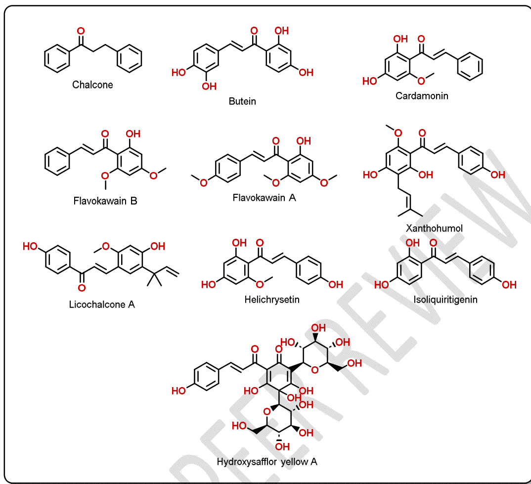
Figure 1: Chalcone and chalcone derived compounds
