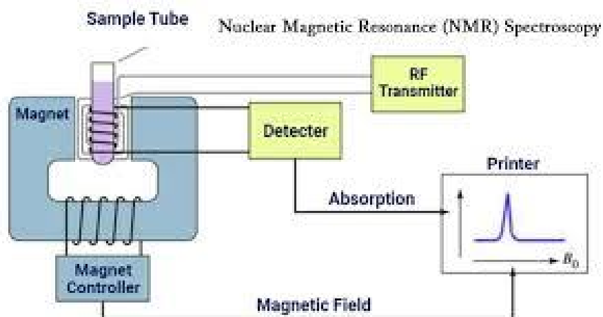
Figure 3: Nuclear Magnetic Resonance (Source: Wikipedia)
