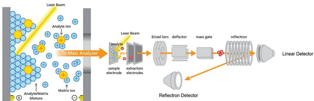
Figure 5: MALDI Technique (Source: Shimadzu)
