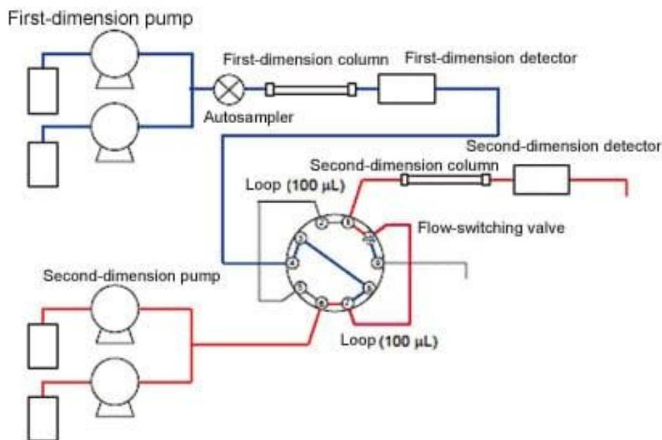
Figure 2: Two-Dimensional High-Performance Liquid Chromatography (2D-HPLC) (Source:Shimadzu)
