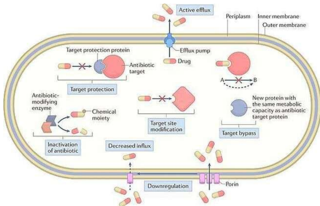
Figure 1. This illustration shows different mechanisms by which bacteria develop resistance to antibiotics [14]
