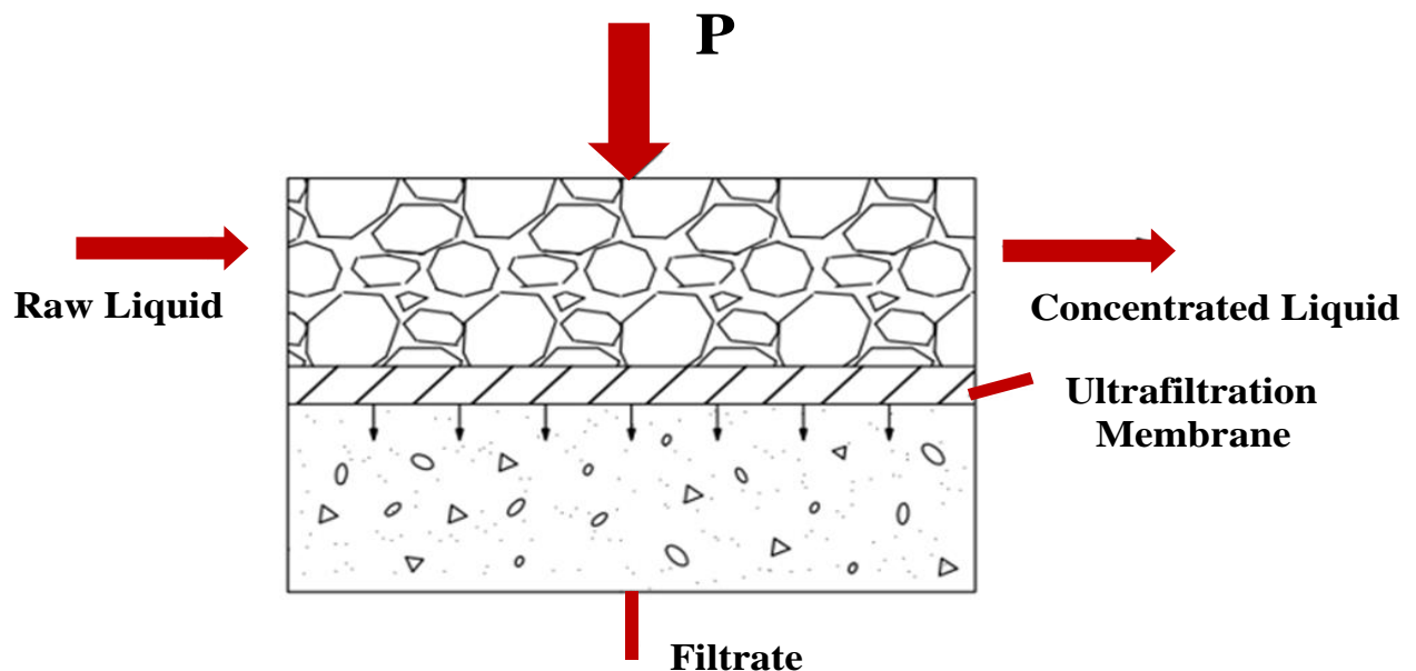
Figure 5. Illustration depicting the ultrafiltration process
