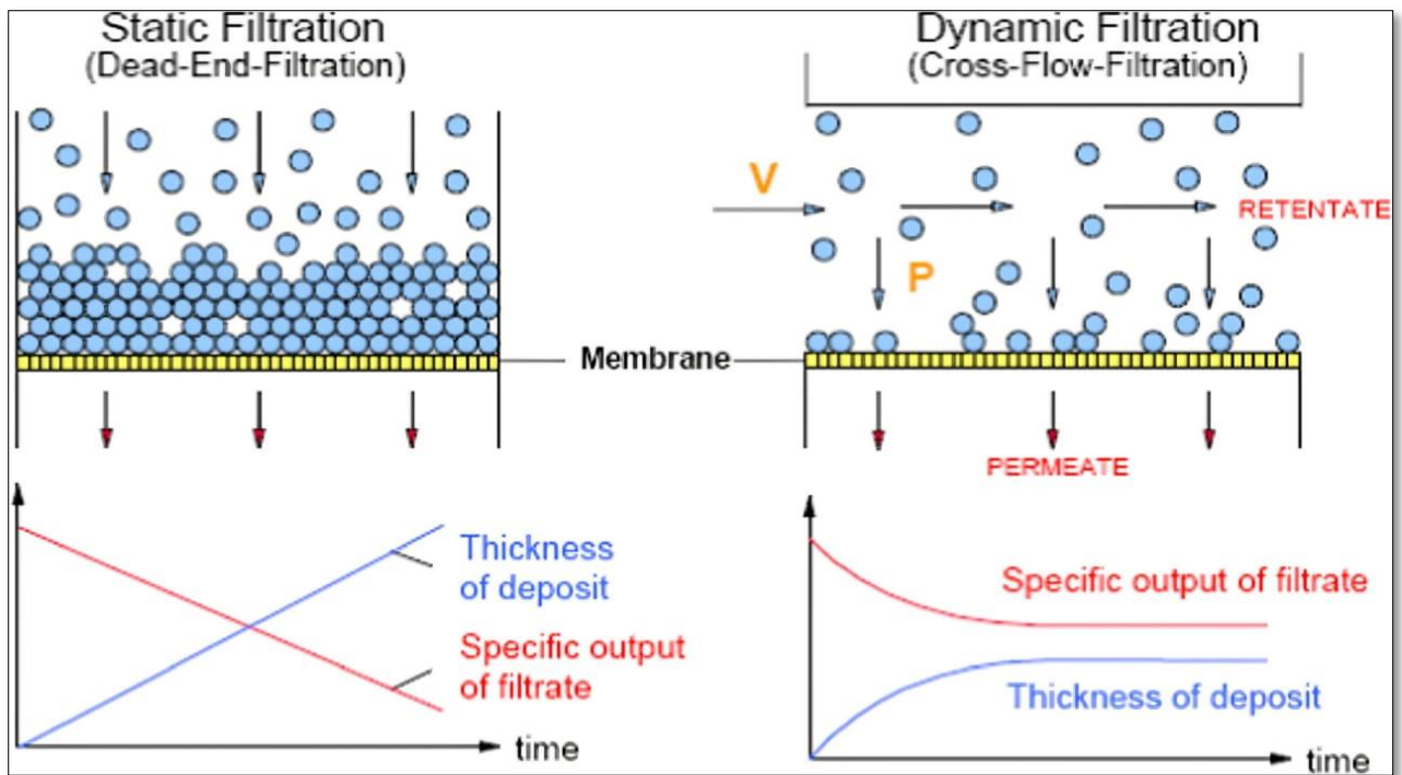
Figure 4: Membrane flow configurations
