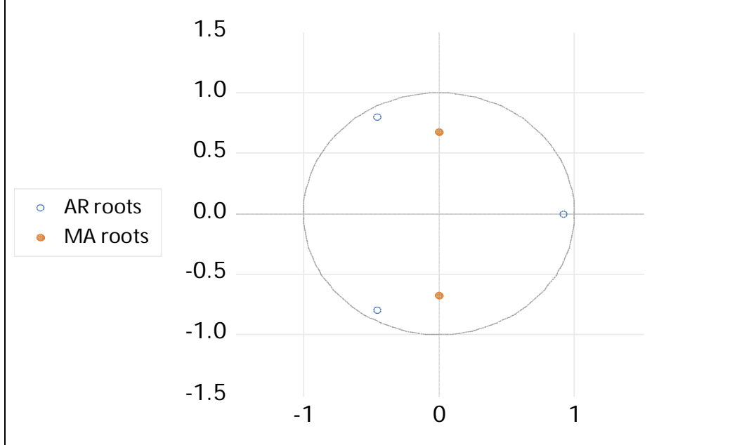
D(BRAEXR): Inverse Roots of AR/MA Polynomial(s)
