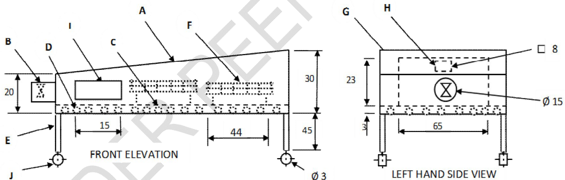
Fig. 1. Schematic representation of the equipment
