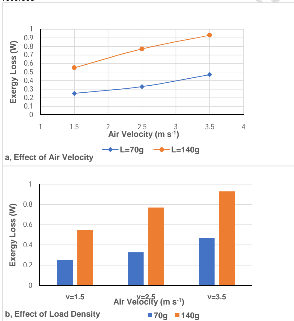
Fig. 3. Effect of air velocity and load density on exergy loss of tiger nut
