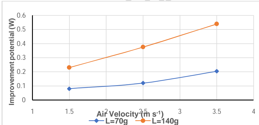
Fig. 6. Effect of air velocity and load density on the improvement potential of tiger nuts
