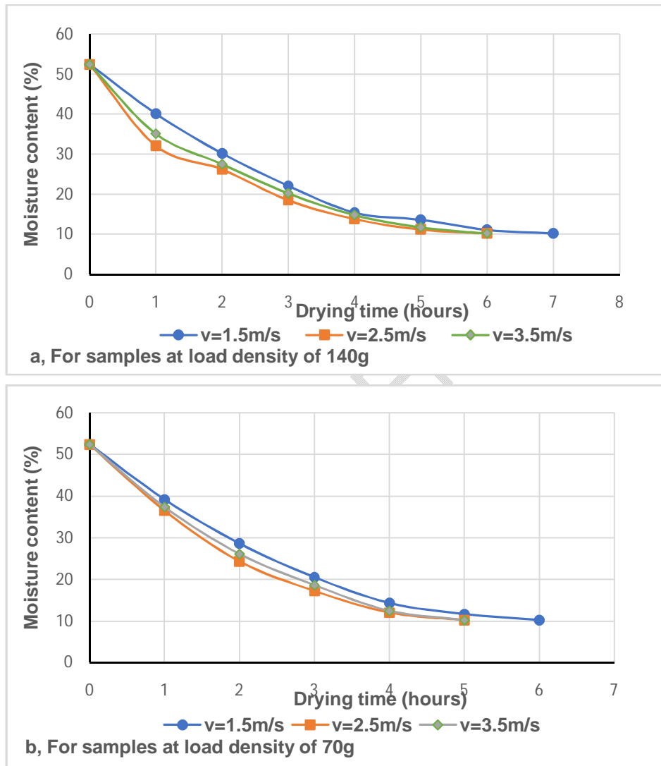
Fig. 7. Moisture desorption curves for the thin-layer drying of tiger nut
