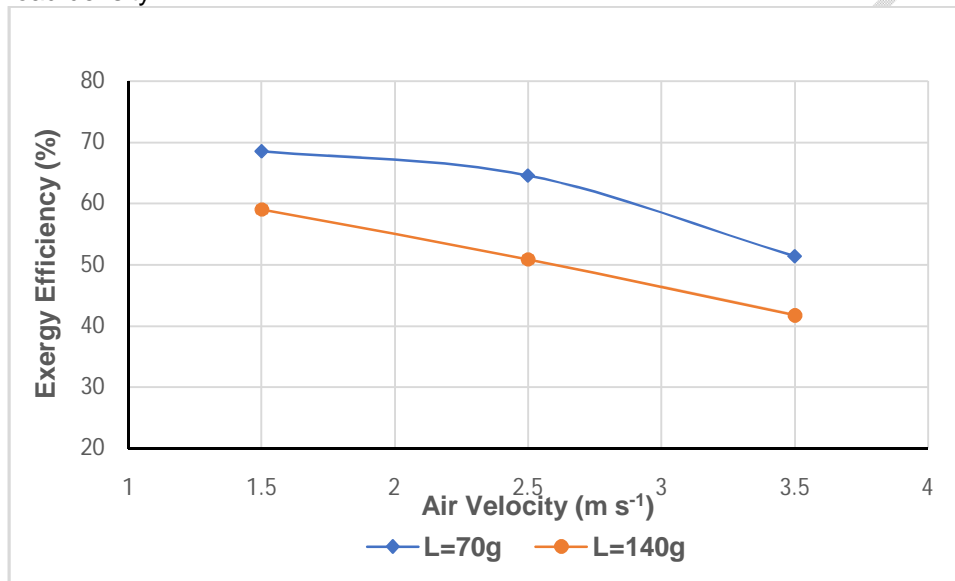
Fig. 4. Effect of air velocity and load density on the exergy efficiency of tiger nuts
