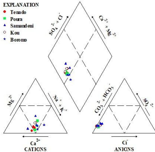
Fig. 4. Piper diagram [88] displaying the dominant water type of the Mouhoun River system
