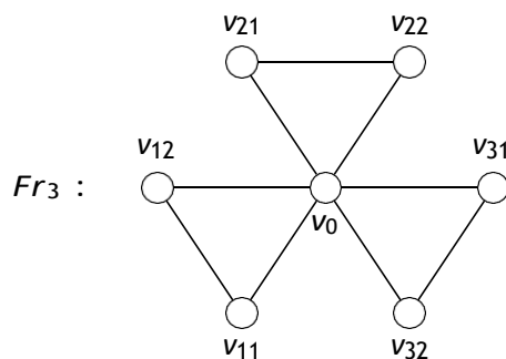
Figure 4: The Friendship Graph Fr_n where n = 3
