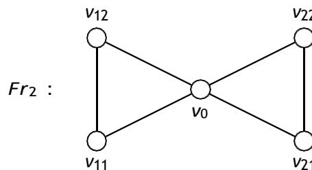
Figure 3: The Friendship Graph Fr_n where n = 2
